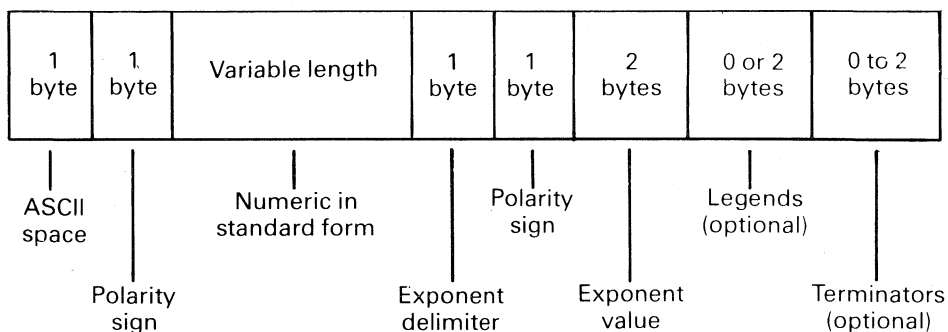
Figure 5.4 Breakdown of a Typical Output String
